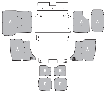
Modelo - Model compact (L0)
